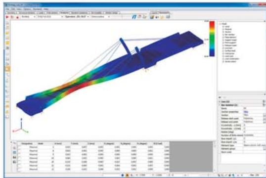
Result for buckling analysis
