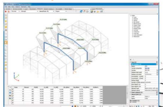
Analysis result illustration for partial model
