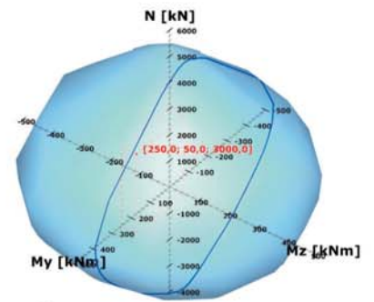
Failure surface for composite cross section
