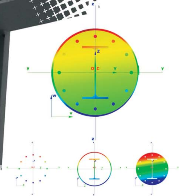
Complex stress distribution on a composite cross section
